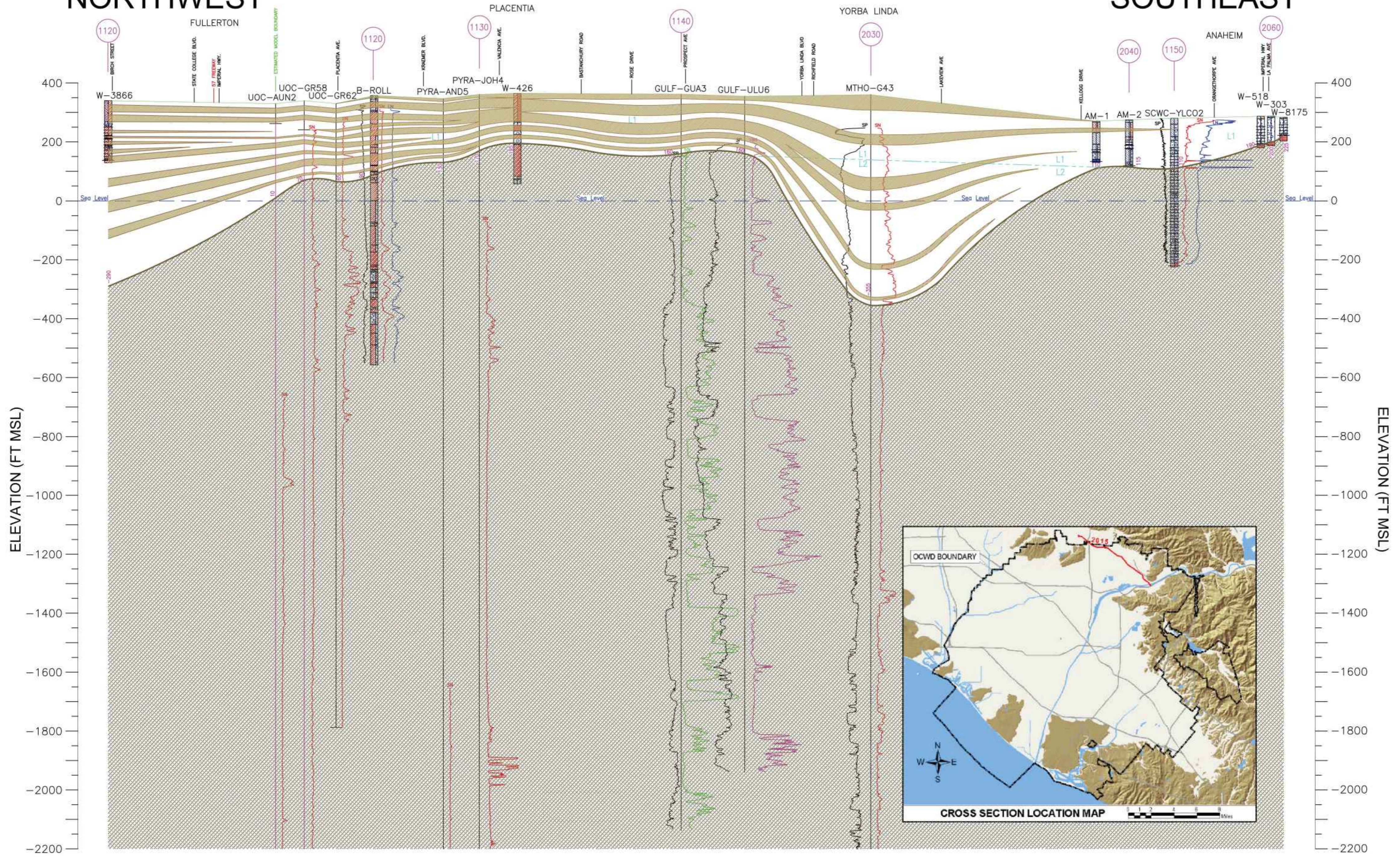
Figure 2-7: Cross Section 2015
