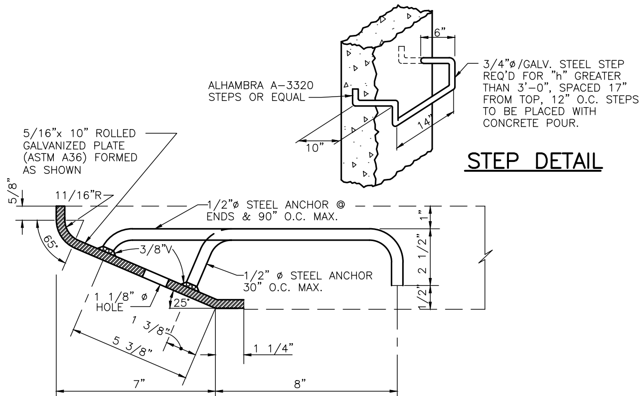
PLATE & ANCHOR DETAIL
