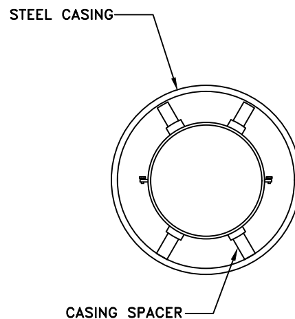
CROSS SECTION
