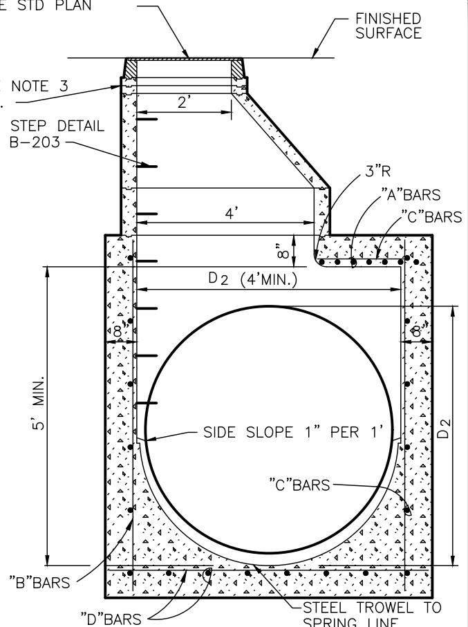
SECTION B-B
