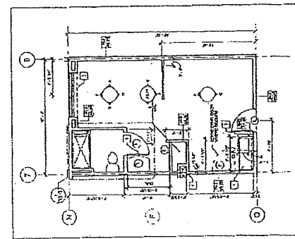
TYPICAL KING SIZE GUEST ROOM SCALE 1/4" = 1'-0"
